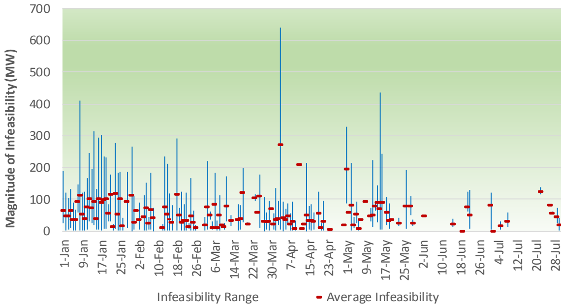
Figure 20: Magnitude of undersupply infeasibility PAC East. Five-minute market.
