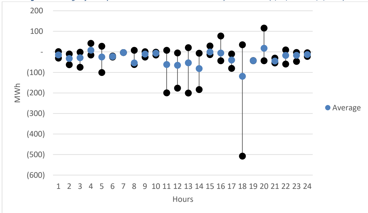
Figure 28: Range of Hourly Undelivered Intertie Resources – Export Direction (8/28/2017 – 9/3/2017)
