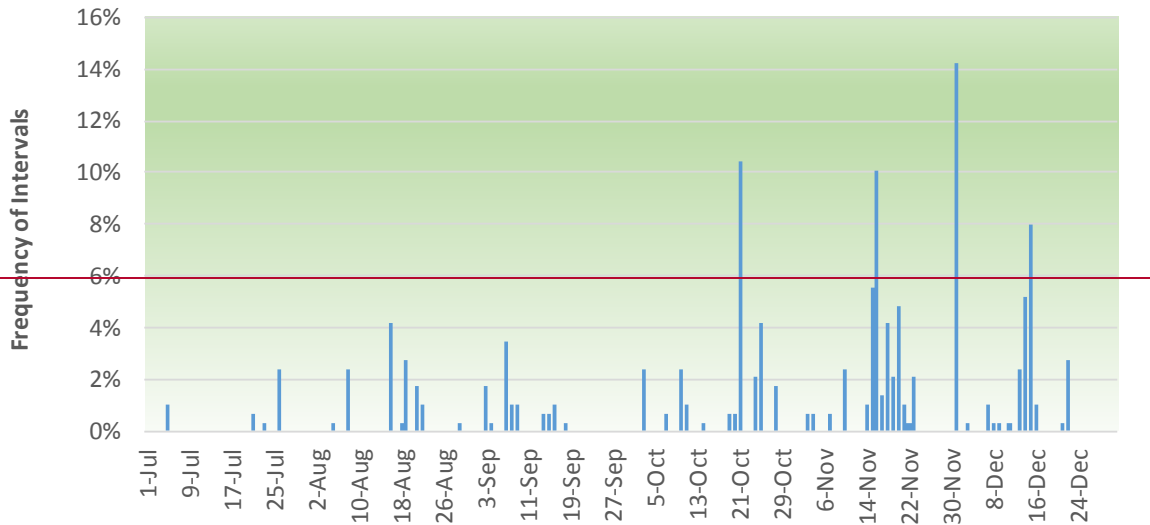
Figure 26: Frequency of oversupply infeasibility PAC West. Five-minute market.
