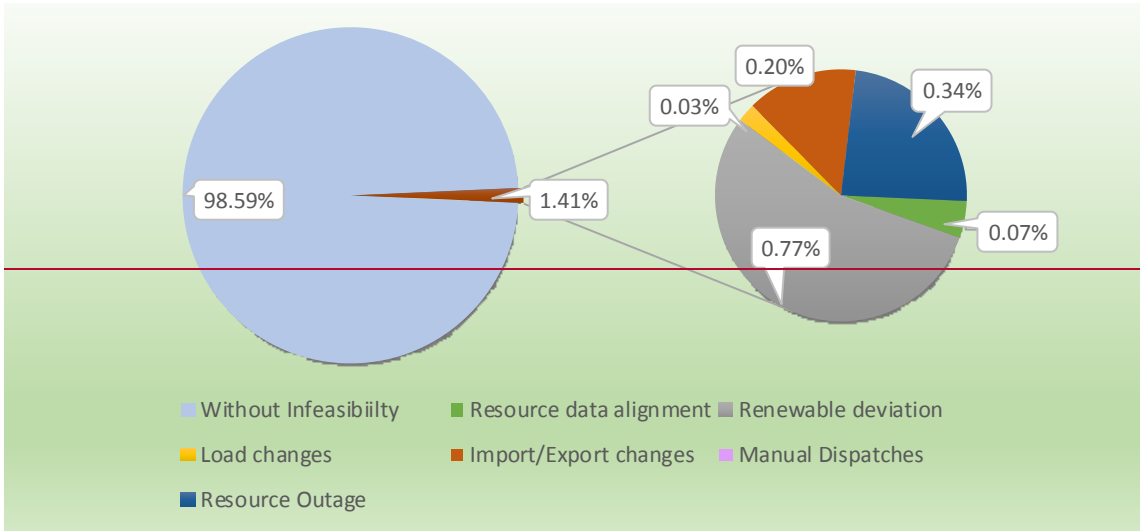
Figure 3: Frequency of undersupply infeasibility in the fifteen-minute market in December January - PAC West and PAC East combined.
