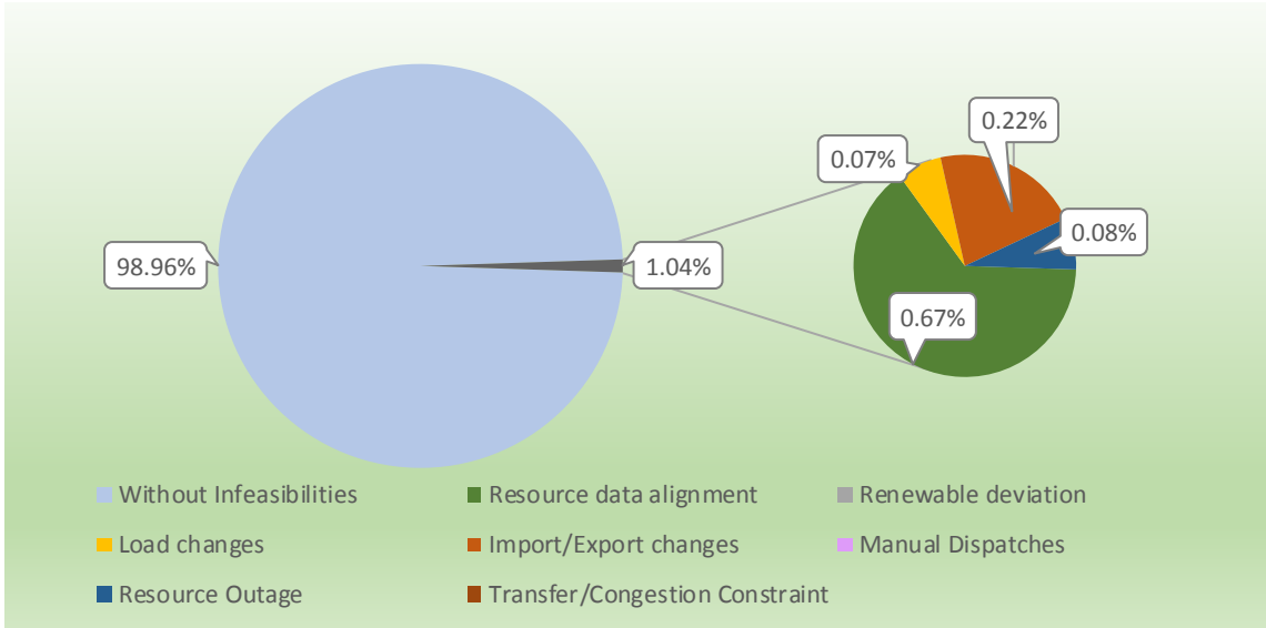
Figure 4: Frequency of undersupply infeasibility in the five-minute market in January - PAC West and PAC East combined.
