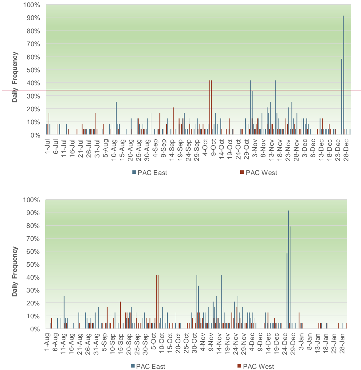
Figure 11: Frequency of balancing test failures in PAC West and East.
